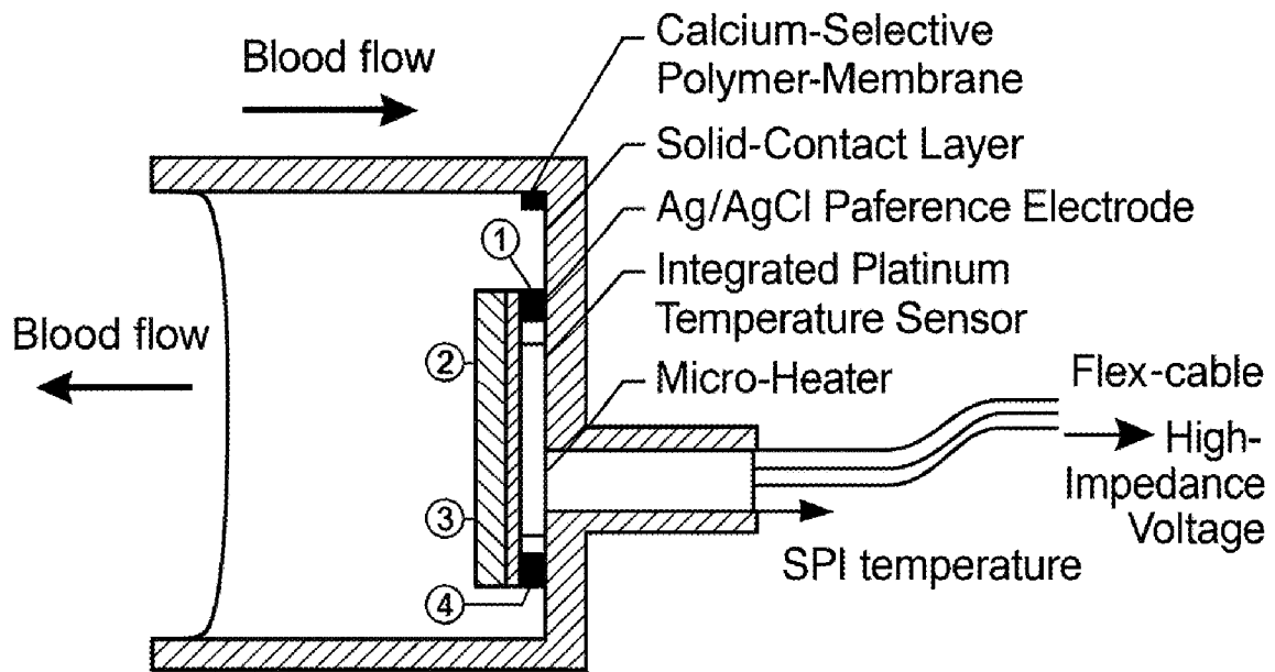
FIG. 4 – Cross-section and signal path of MEMS inline ion-selective calcium sensor (505/506)
