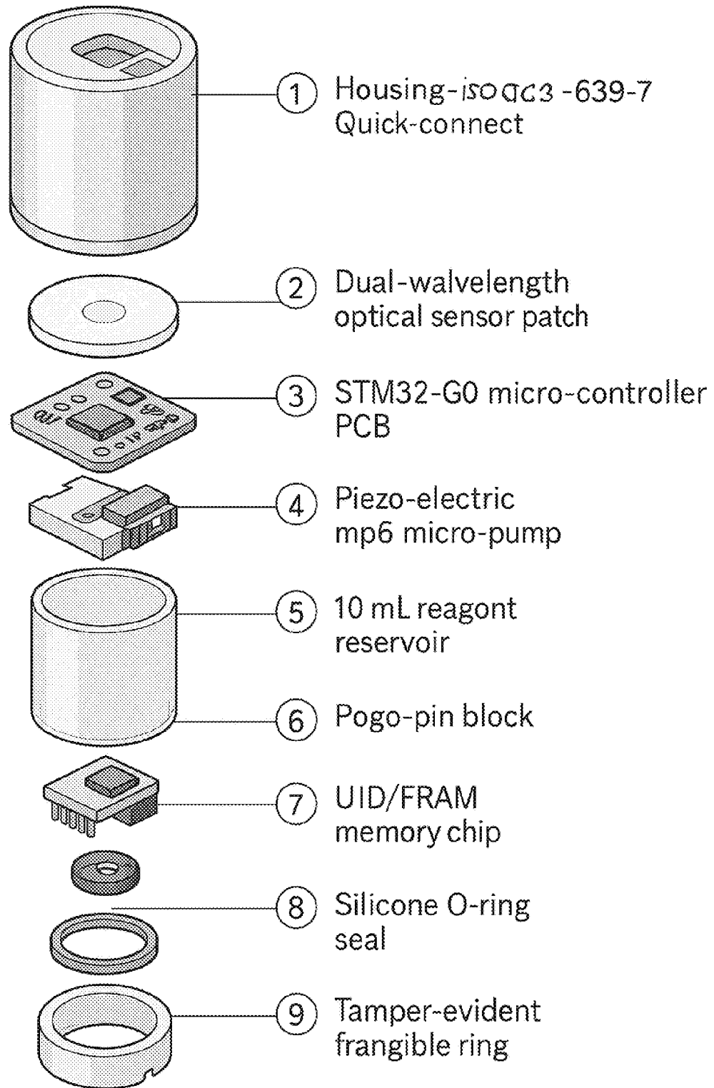
Exploded-isometric transct cartridge
