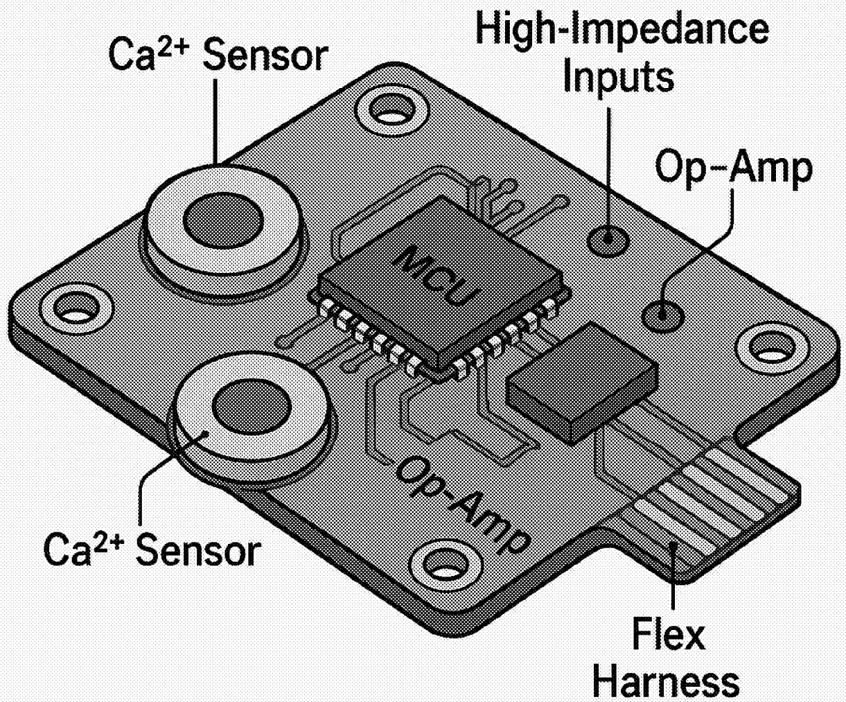
Sensor Board Layout
