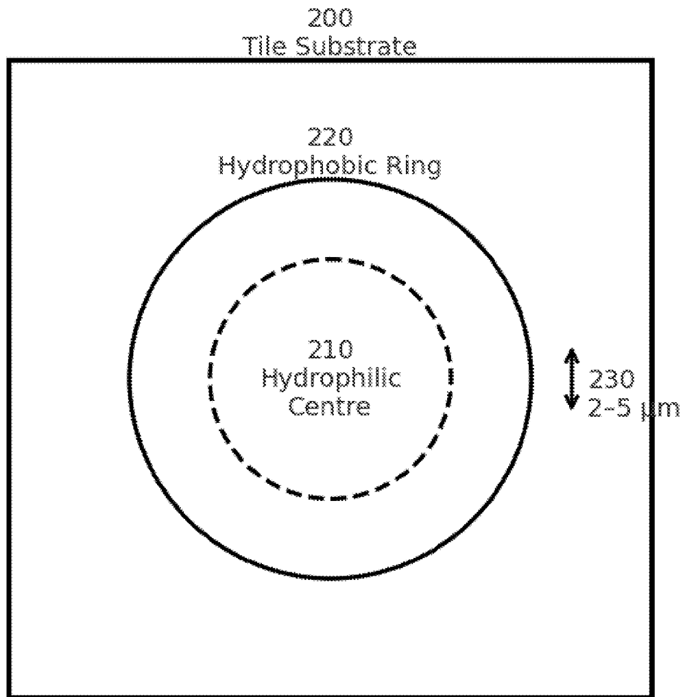
FIG. 2 - Disposable Serum-Tile Geometry
