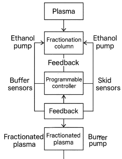
Figure 2 Batch Execution and Sensor Feedback Flowchart
