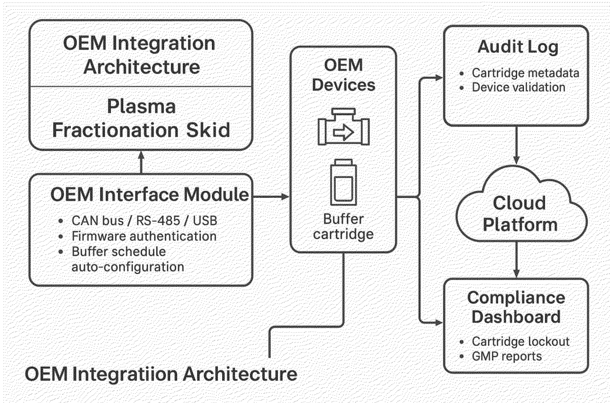
FIGURE 4: OEM Integration Architecture for Plasma Fractionation
