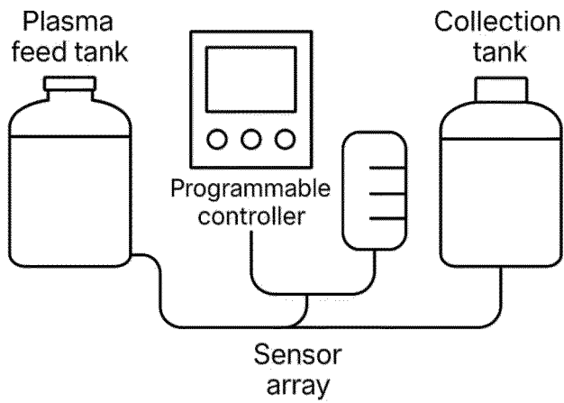
Figure 1 Sensor-Integrated Skid Modules for Inline Detection
