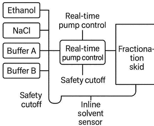
Figure 3 Modular Ethanol and Buffer Dosing Pumps System
